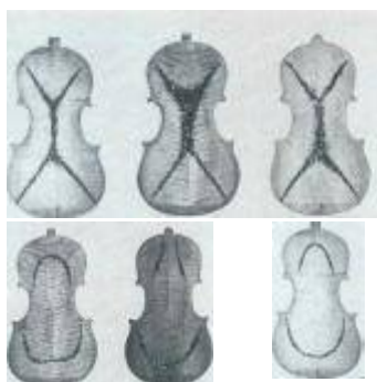
WELL-TUNED AND POORLY TUNED PLATES are revealed by means of the Chladni technique. Each pair of photographs, top and bottom, shows modes 2 and 5 respectively of a violin back plate. In the plate at the left both modes are well tuned. In the plate at the center the nodal areas of mode 2 are too wide in the upper section, indicating that the entire upper area of the plate is too stiff. In the plate at the right the nodal areas of mode 5 extend straight to the upper edge instead of closing into a ring shape. This usually happens when the plates are too thick through the upper section of the center between the C-bouts and inside the upper corner.
