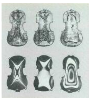
TWO TECHNIQUES for demonstrating the eigenmodes of a free violin plate are compared. In the photographs at the top the Chladni patterns of a back plate are shown at frequencies of 165, 225 and 357 hertz. Laser interferograms of the same plate at a different relative humidity are shown in the photographs at the bottom at frequencies of 165, 222 and 348 hertz. The nodal patterns, which show in the interferograms as wide white areas, are indicated by the quite similar dark shapes in the Chladni patterns. The laser technique not only is more sensitive than the Chladni one to small vibrations of a top or back plate but also indicates motion in the anti-nodal areas of a plate by the narrow and dark lines of the characteristic interference fringes.
